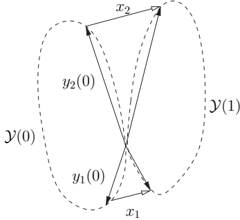
Figure 2: This picture illustrates for the case p = 2 , n = 3 how \xi_{\circ Y} represents an “elementary variation” \xi of the subspace \mathcal{Y} spanned by the columns of Y . Consider Y(0) = [y_1(0)|y_2(0)] and \xi_{\circ Y(0)} = [x_1|x_2] . By the horizontality condition Y(0)^T \xi_{\circ Y(0)} = 0 , both x_1 and x_2 are normal to the space \mathcal{Y}(0) spanned by Y(0) . Let y_1(t) = y_1(0) + tx_1 , y_2(t) = y_2(0) + tx_2 and let \mathcal{Y}(t) be the subspace spanned by y_1(t) and y_2(t) . Then we have \xi = \dot{\mathcal{Y}}(0) .
